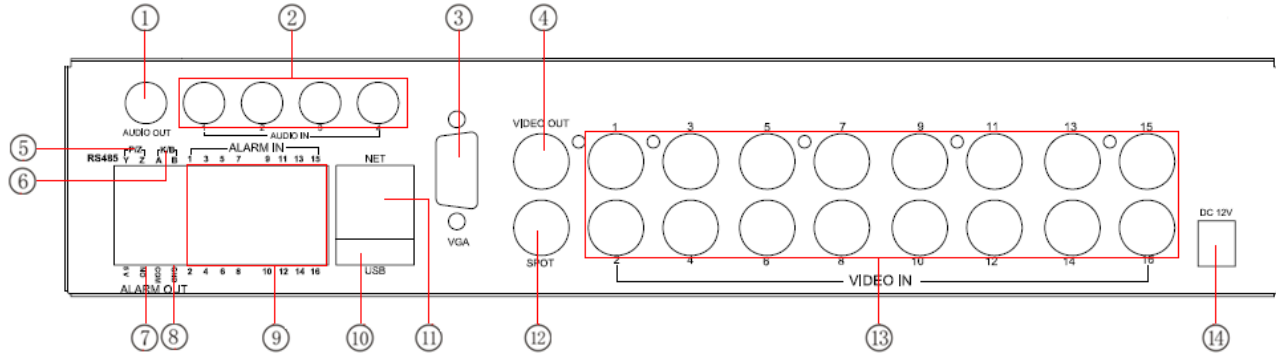
Fig 2.6 Rear Panel for 16-ch
