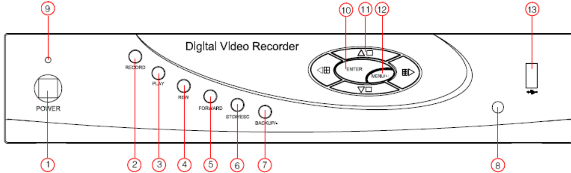
Fig 2.3 Front Panel
