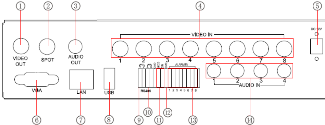
Fig 2.5 Rear Panel for 8-ch
